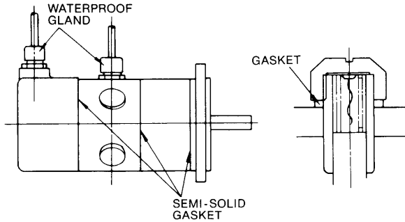
Fig. 8 Drip-proof Enclosure
