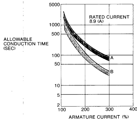
Fig. 2 Starting and Overload Characteristics
