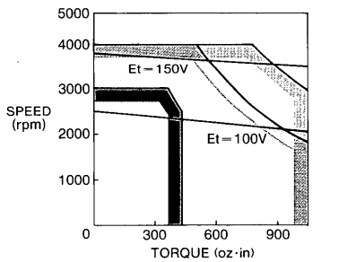
Fig. 1 Speed-Torque Characteristics
