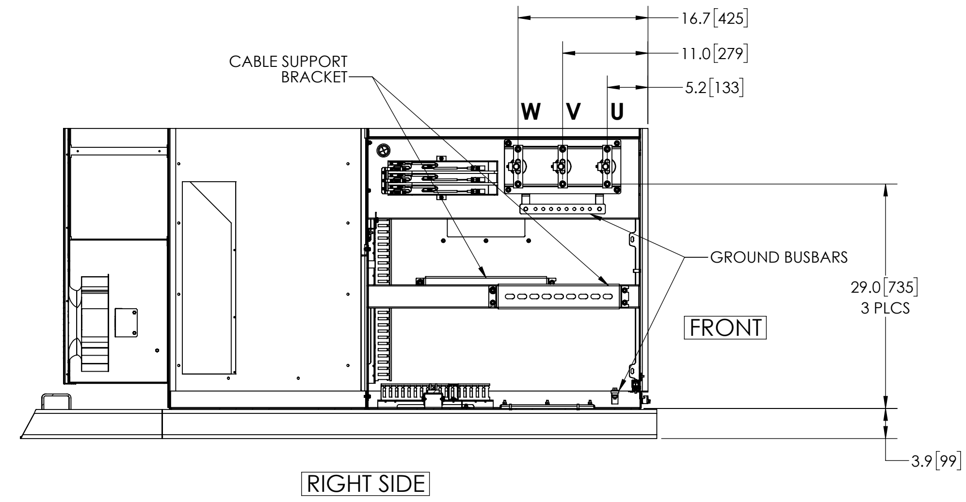
OUTPUT TERMINAL LOCATIONS SECTION E-E
