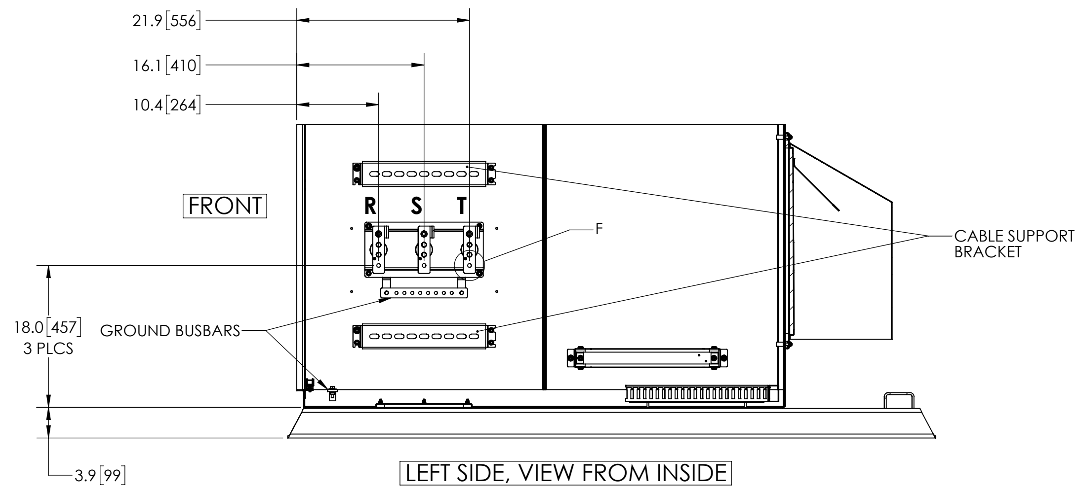
INPUT TERMINAL LOCATIONS SECTION D-D
